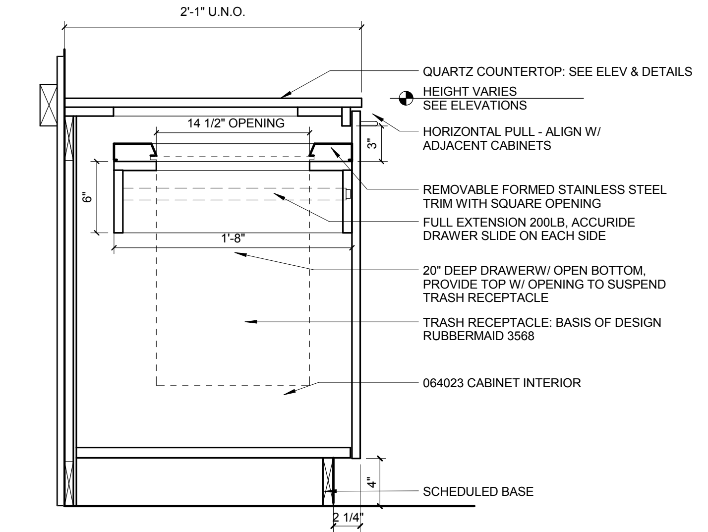
3 BASE CABINET WASTE DRAWER 1 1/2" = 1'-0"
