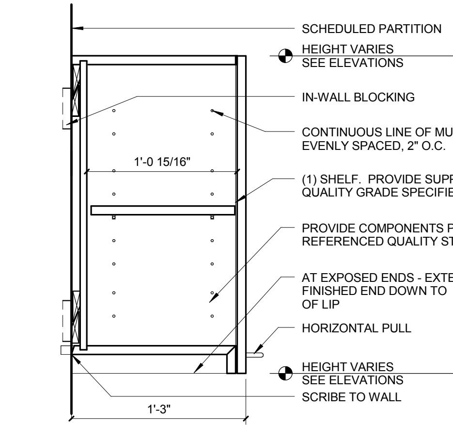
7 UPPER CABINET 1 1/2" = 1'-0"
